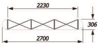
3 x 3 - Straight
